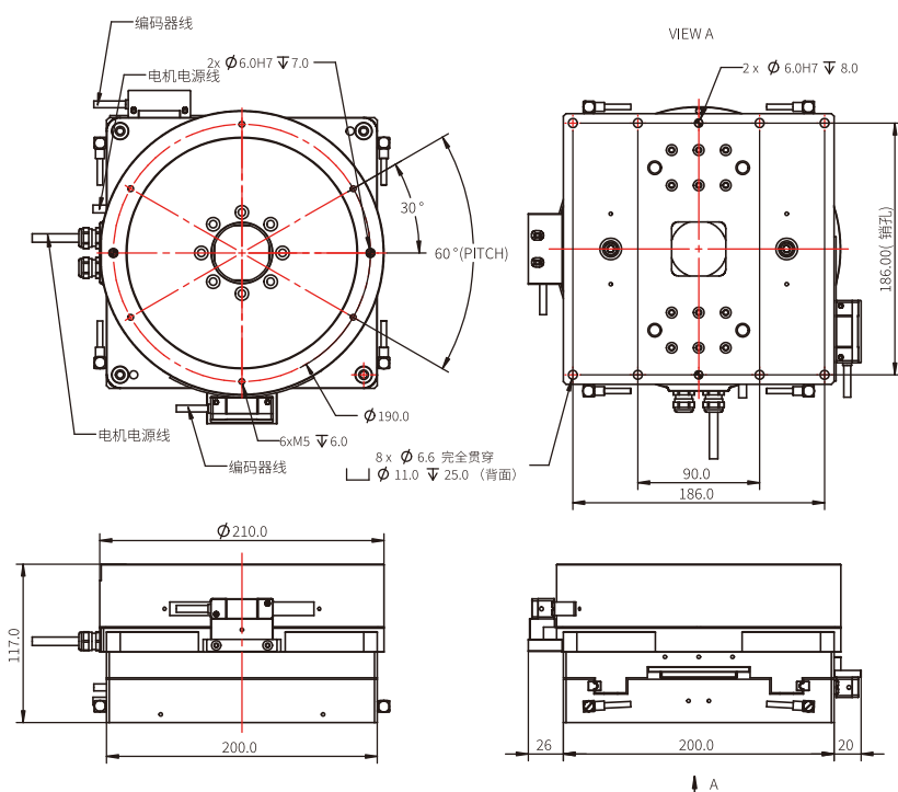
TYSM-200S-X20T20-CJ10-0.5对位机器人/TYSM-200S-X20T20-CJ10-0.5 Alignment Stage
