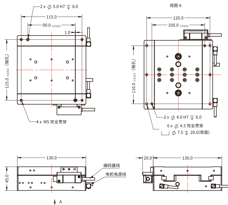
TYSM-130S-X20-CJ10-0.5对位机器人/TYSM-130S-X20-CJ10-0.5 Alignment Stage
