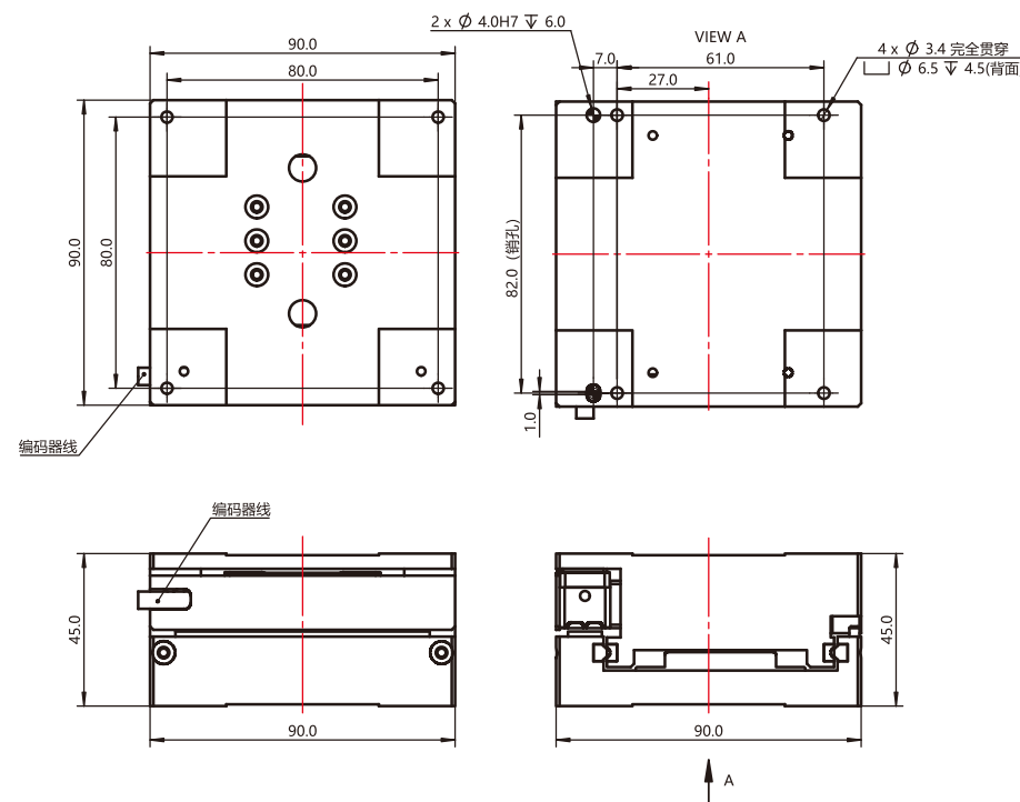
TYSM-90S-X15-CJ10-0.5对位机器人/TYSM-90S-X15-CJ10-0.5 Alignment Stage
