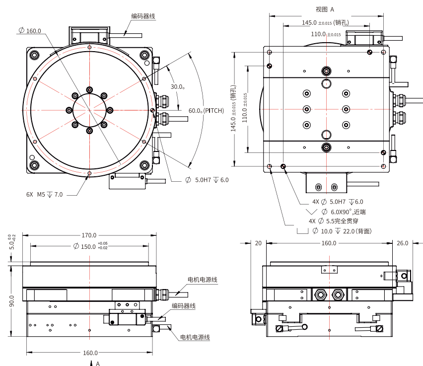
TYSM-160S-X30T15-CJ10-0.5对位机器人/TYSM-160S-X30T15-CJ10-0.5 Alignment Stage
