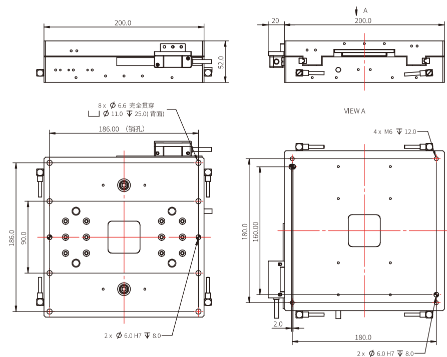
TYSM-200S-X20-CJ10-0.5对位机器人/TYSM-200S-X20-CJ10-0.5 Alignment Stage
