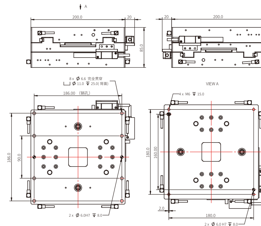
TYSM-200S-XY20-CJ10-0.5对位机器人/TYSM-200S-XY20-CJ10-0.5 Alignment Stage
