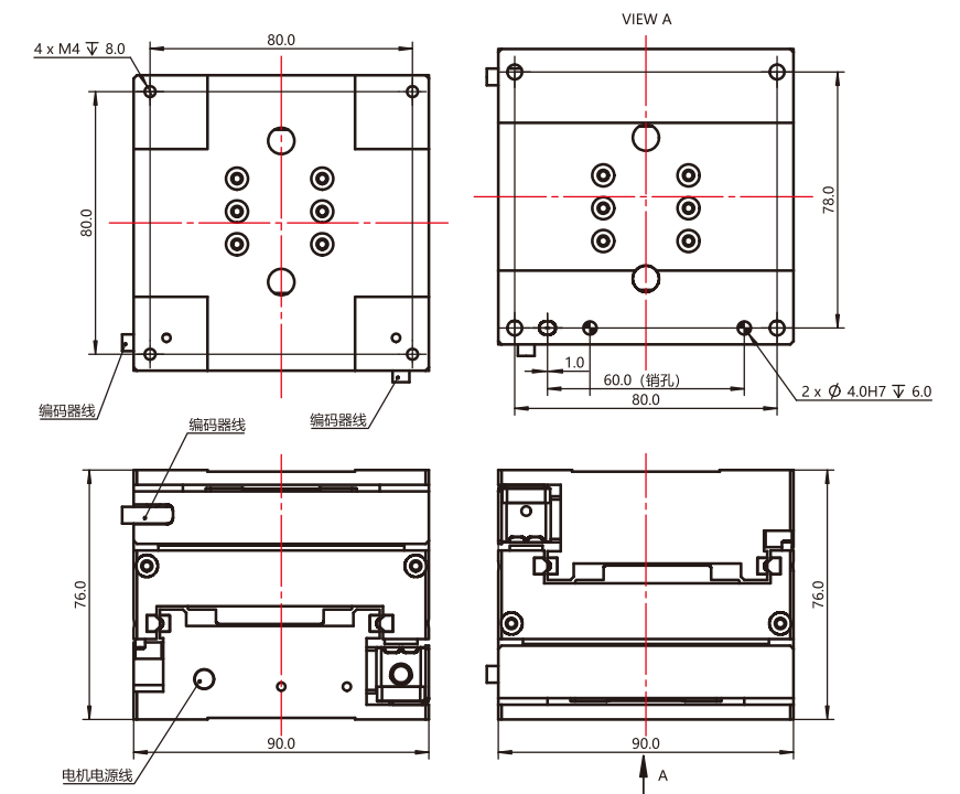
TYSM-90S-X15-CJ10-0.5对位机器人/TYSM-90S-XY15-CJ10-0.5 Alignment Stage
