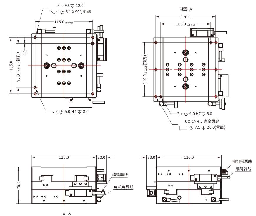
TYSM-130S-XY20-CJ10-0.5对位机器人/TYSM-130S-XY20-CJ10-0.5 Alignment Stage
