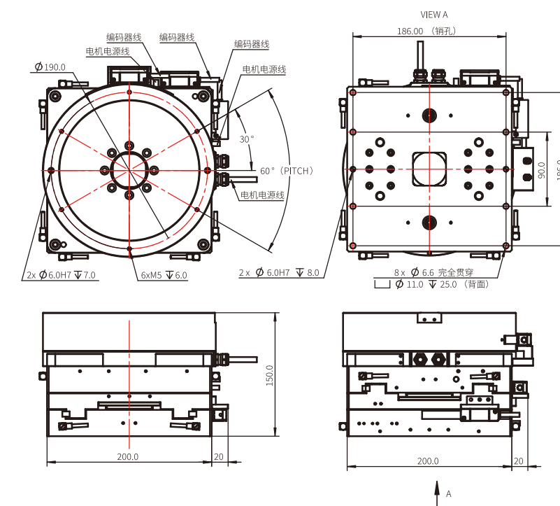
TYSM-200S-XY20T20-CJ10-0.5对位机器人/TYSM-200S-XY20T20-CJ10-0.5 Alignment Stage
