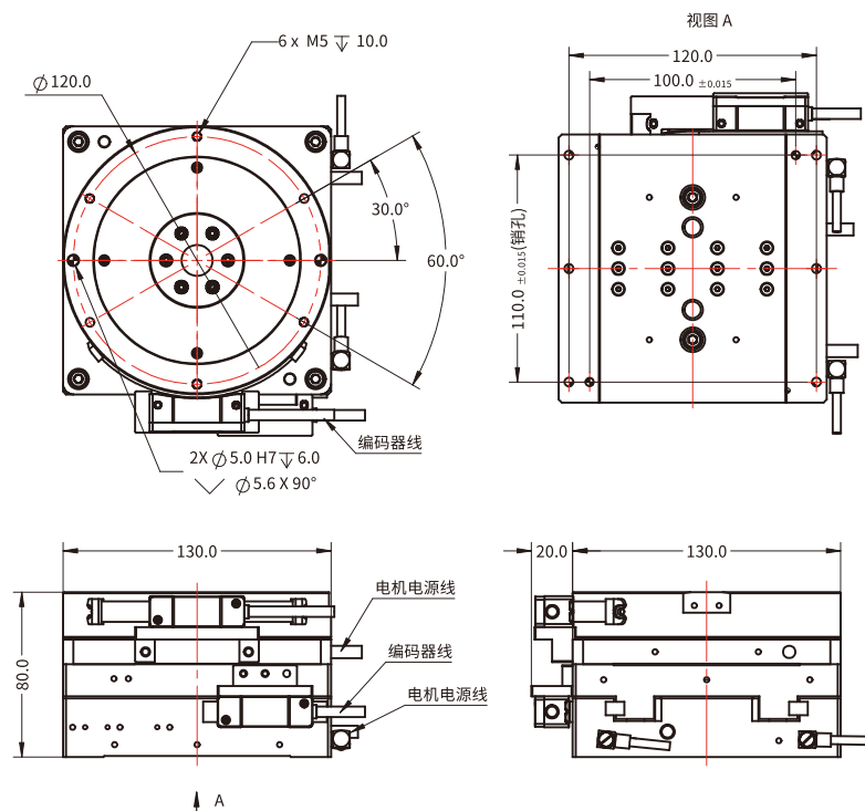
TYSM-130S-X20T10-CJ10-0.5对位机器人/TYSM-130S-X20T10-CJ10-0.5 Alignment Stage
