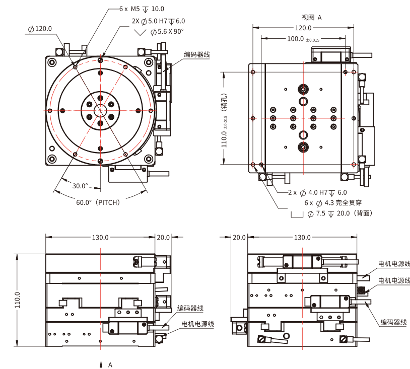
TYSM-130S-XY20T10-CJ10-0.5对位机器人/TYSM-130S-XY20T10-CJ10-0.5 Alignment Stage
