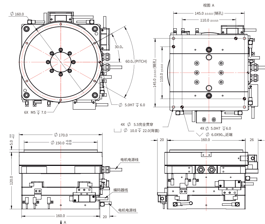
TYSM-160S-XY30T15-CJ10-0.5对位机器人/TYSM-160S-XY30T15-CJ10-0.5 Alignment Stage
