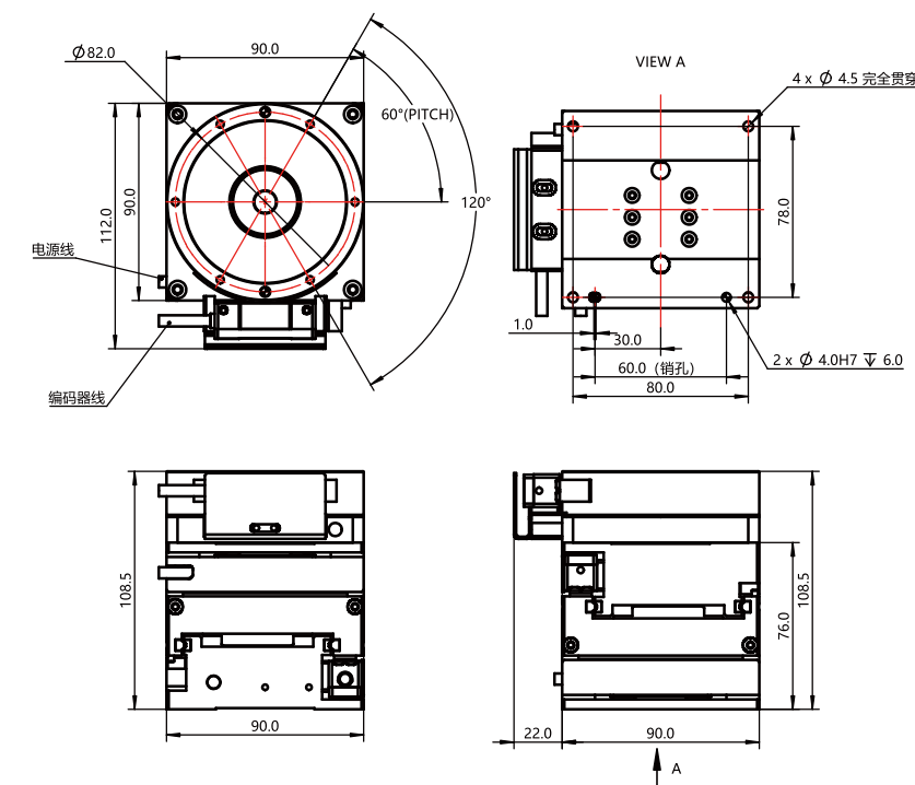
TYSM-90S-X15T10-CJ10-0.5对位机器人/TYSM-90S-XY15-CJ10-0.5 Alignment Stage
