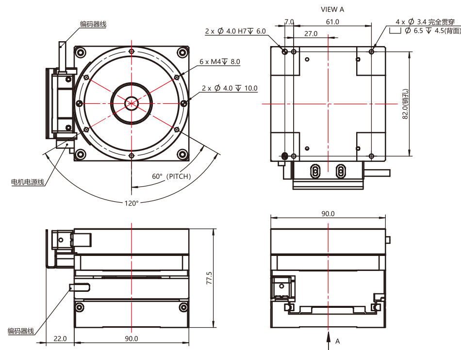
TYSM-90S-X15T10-CJ10-0.5对位机器人/TYSM-90S-X15-CJ10-0.5 Alignment Stage
